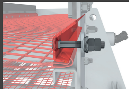
SCREW FASTENING
